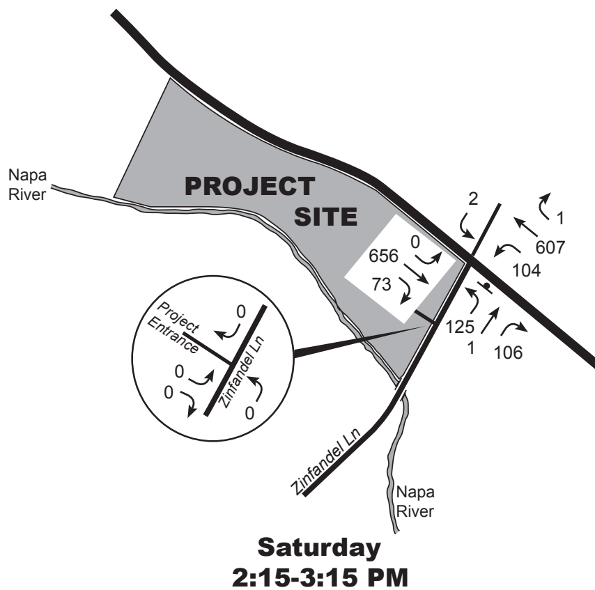
Figure 5 Year 2018 without Project (Harvest) Friday and Saturday PM Peak Hour Volumes
