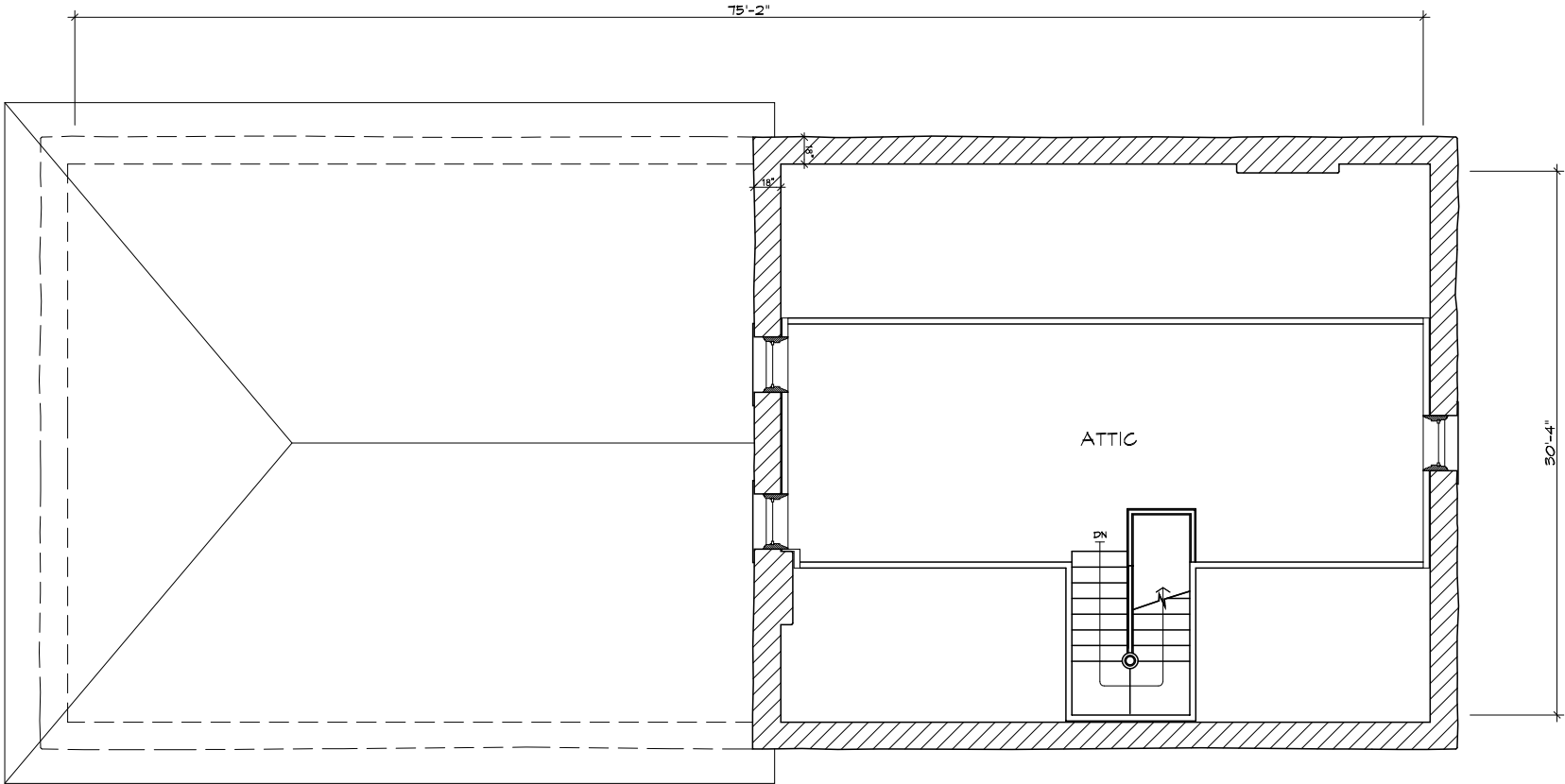
A ATTIC (THIRD) FLOOR PLAN
