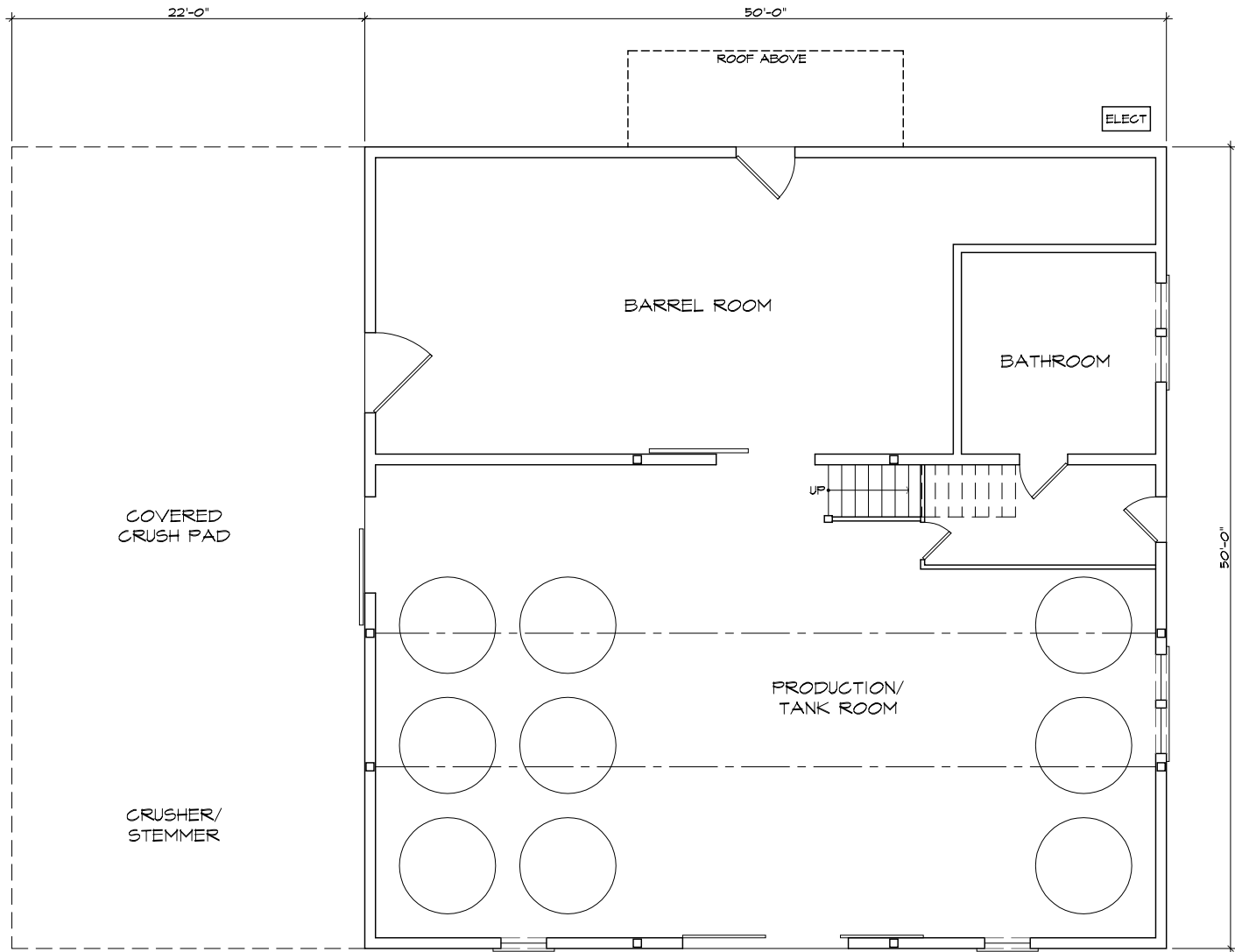
A FIRST FLOOR PLAN
