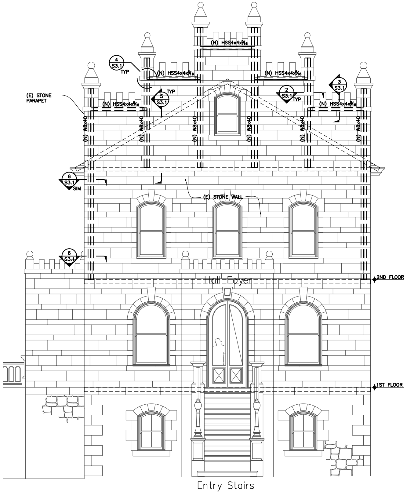
1 BUILDING ELEVATION S3.1
