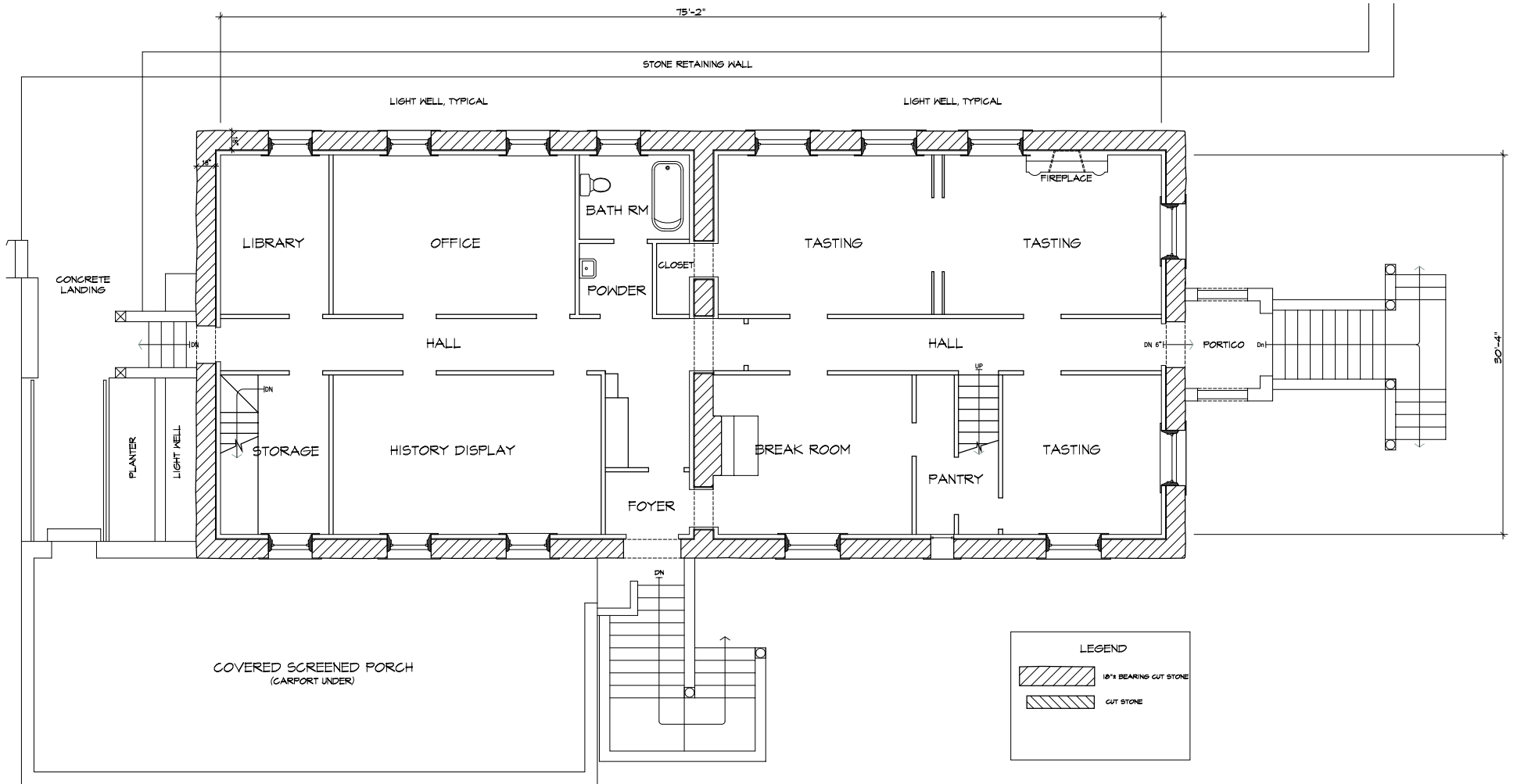
A FIRST FLOOR PLAN
